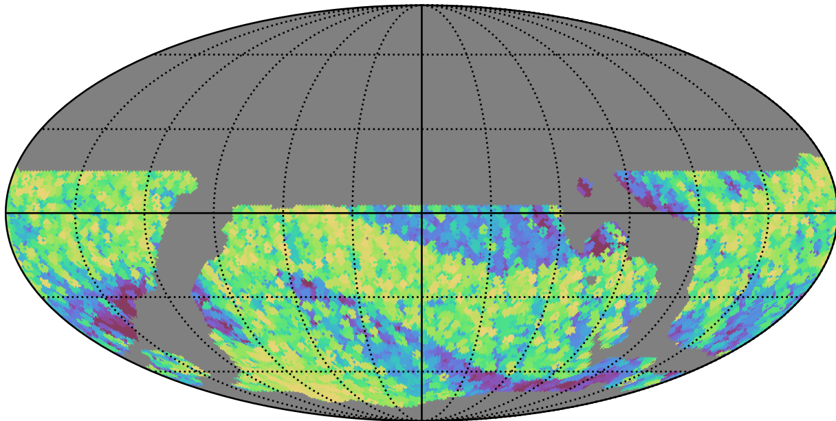
weather_cloudso12v3.4_10yrs WFD all bands: Max airmass
