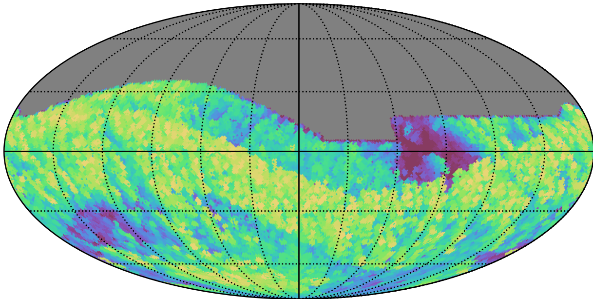
weather_cloudso12v3.4_10yrs All sky z band: Max airmass
