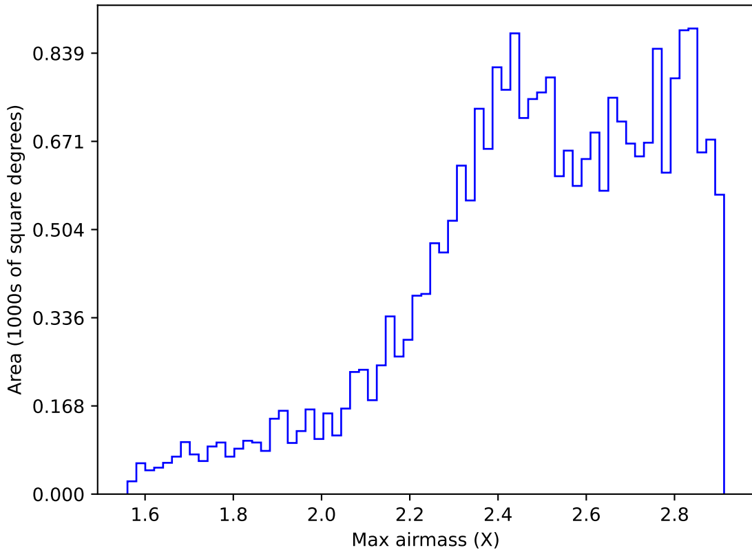
weather_cloudso12v3.4_10yrs All sky z band: Max airmass
