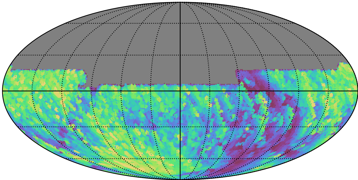
weather_cloudso12v3.4_10yrs All sky y band: Max airmass
