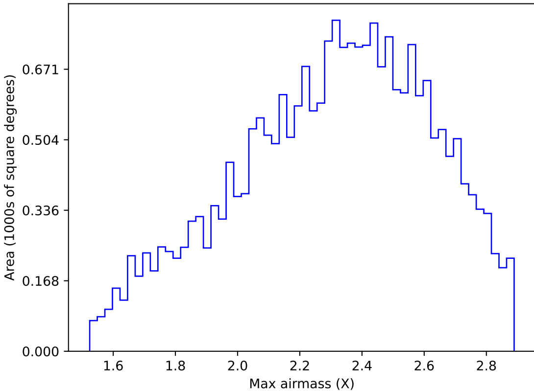
weather_cloudso12v3.4_10yrs All sky y band: Max airmass
