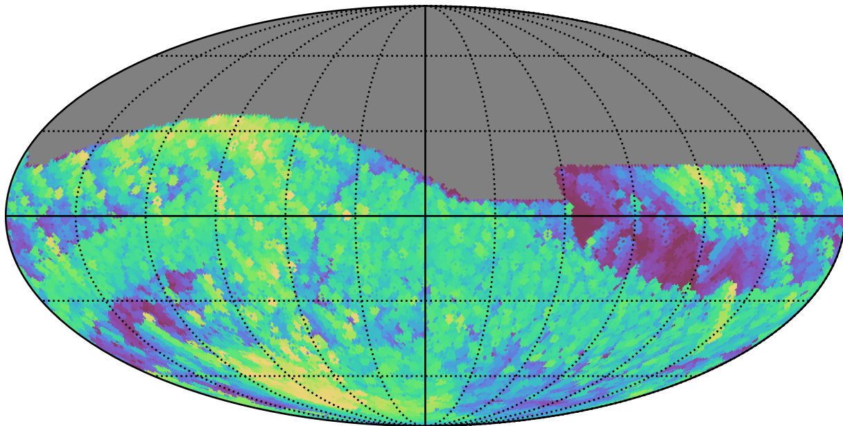
weather_cloudso12v3.4_10yrs All sky r band: Max airmass
