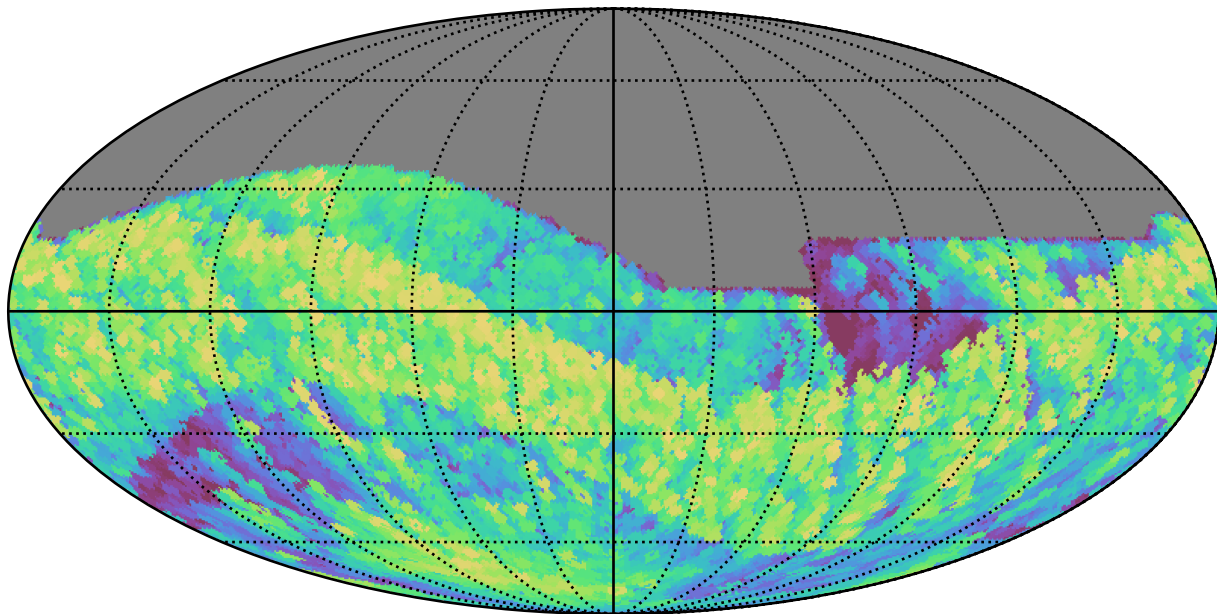
weather_cloudso12v3.4_10yrs All sky i band: Max airmass
