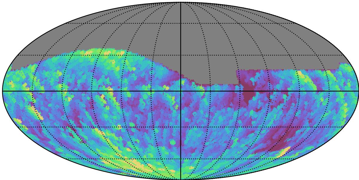
weather_cloudso12v3.4_10yrs All sky g band: Max airmass
