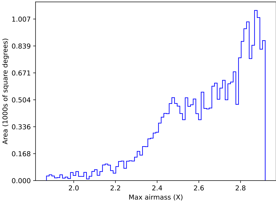
weather_cloudso12v3.4_10yrs All sky all bands: Max airmass
