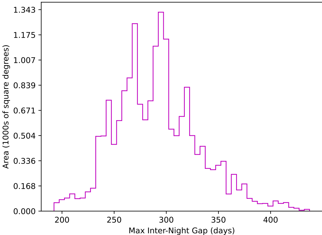
weather_cloudso12v3.4_10yrs WFD z band: Max Inter-Night Gap
