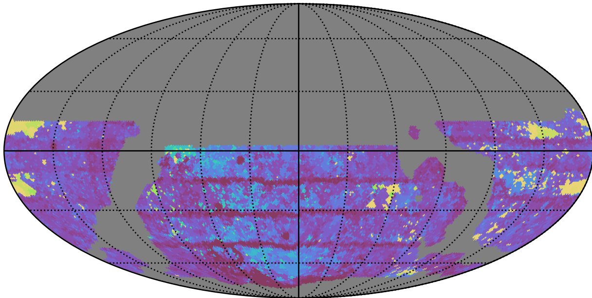
weather_cloudso12v3.4_10yrs WFD y band: Max Inter-Night Gap
