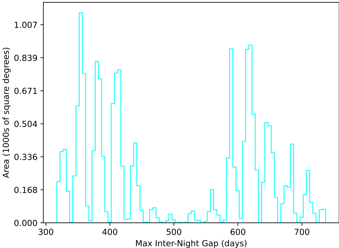
weather_cloudso12v3.4_10yrs WFD u band: Max Inter-Night Gap
