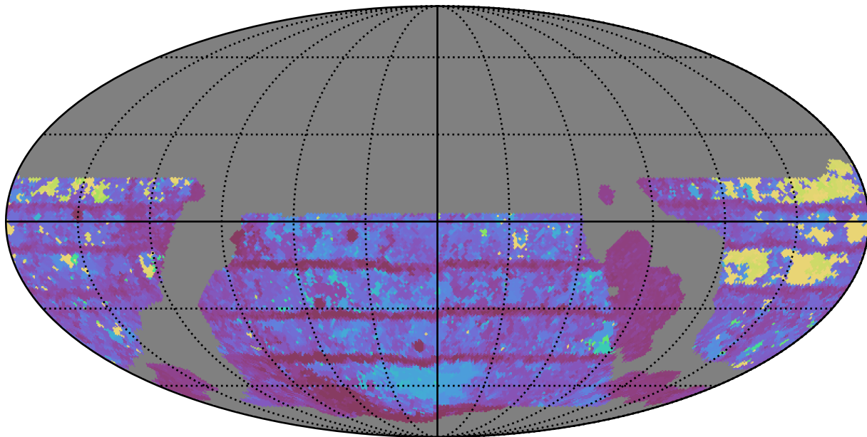
weather_cloudso12v3.4_10yrs WFD r band: Max Inter-Night Gap
