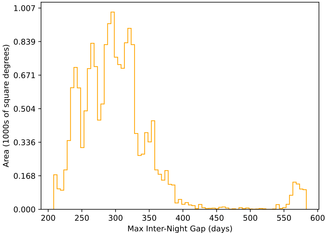
weather_cloudso12v3.4_10yrs WFD r band: Max Inter-Night Gap
