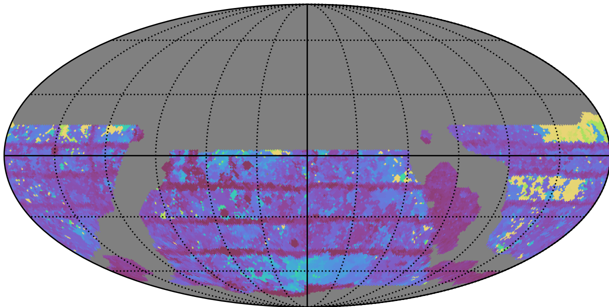
weather_cloudso12v3.4_10yrs WFD i band: Max Inter-Night Gap
