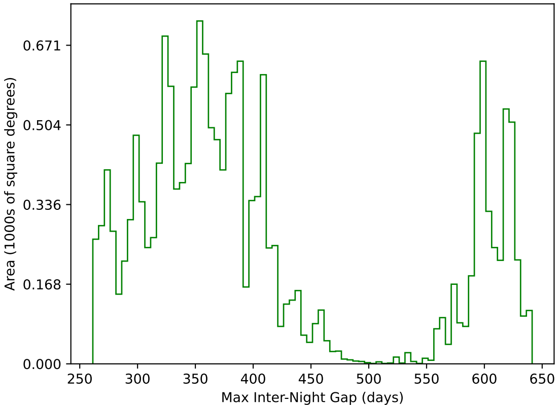
weather_cloudso12v3.4_10yrs WFD g band: Max Inter-Night Gap
