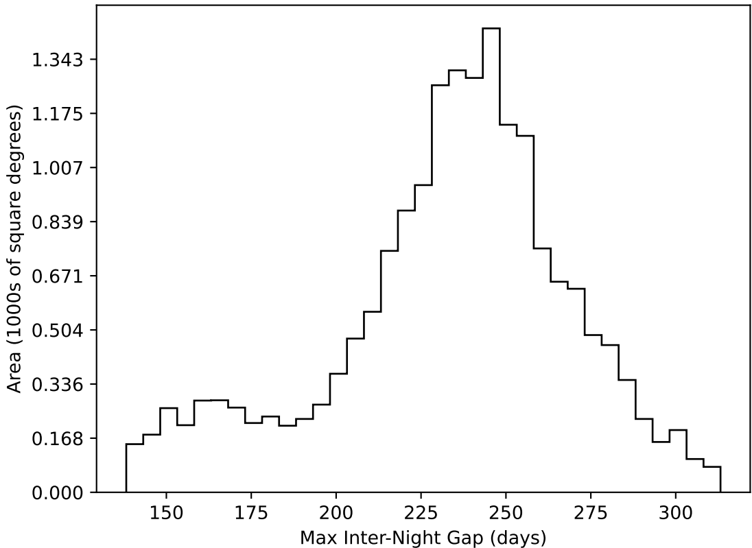
weather_cloudso12v3.4_10yrs WFD all bands: Max Inter-Night Gap
