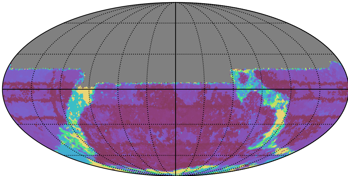
weather_cloudso12v3.4_10yrs All sky u band: Max Inter-Night Gap
