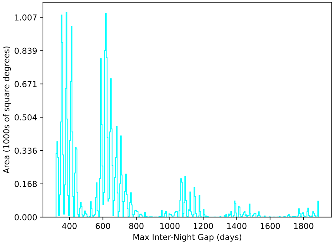
weather_cloudso12v3.4_10yrs All sky u band: Max Inter-Night Gap
