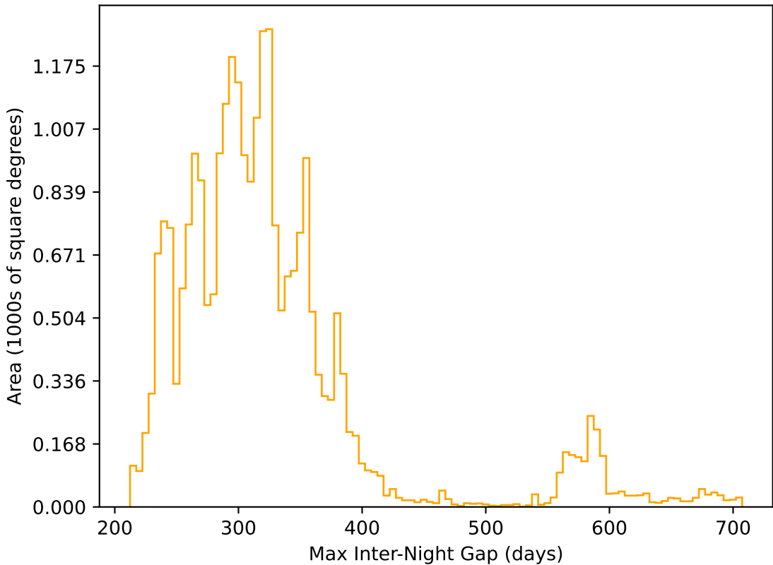
weather_cloudso12v3.4_10yrs All sky r band: Max Inter-Night Gap
