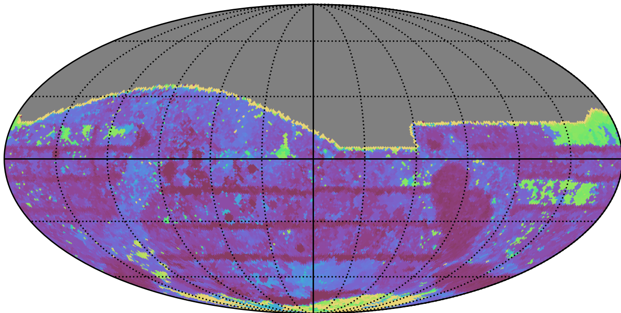
weather_cloudso12v3.4_10yrs All sky i band: Max Inter-Night Gap
