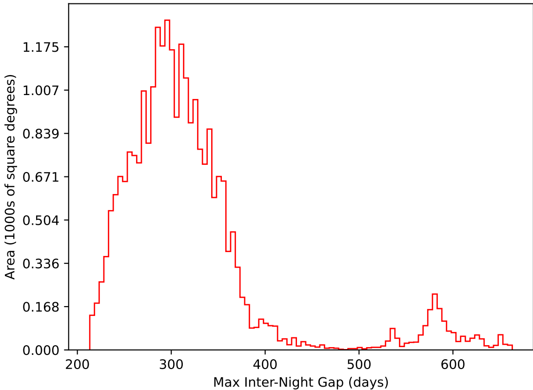
weather_cloudso12v3.4_10yrs All sky i band: Max Inter-Night Gap
