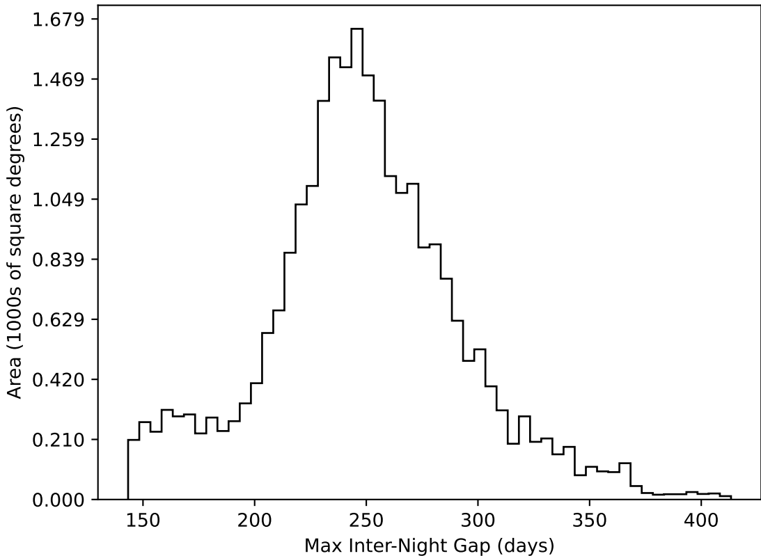
weather_cloudso12v3.4_10yrs All sky all bands: Max Inter-Night Gap
