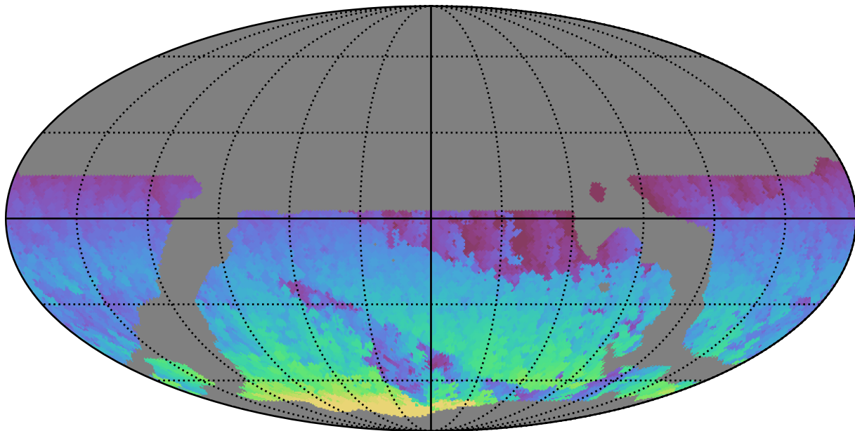
weather_cloudso12v3.4_10yrs WFD z band: Max HA
