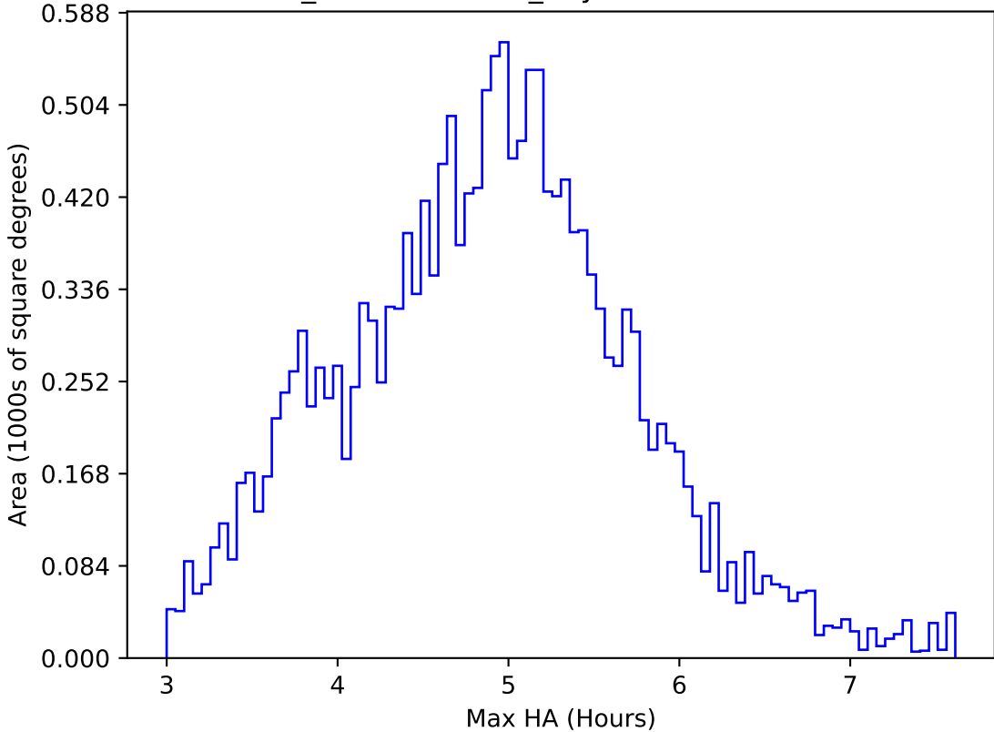
weather_cloudso12v3.4_10yrs WFD z band: Max HA
