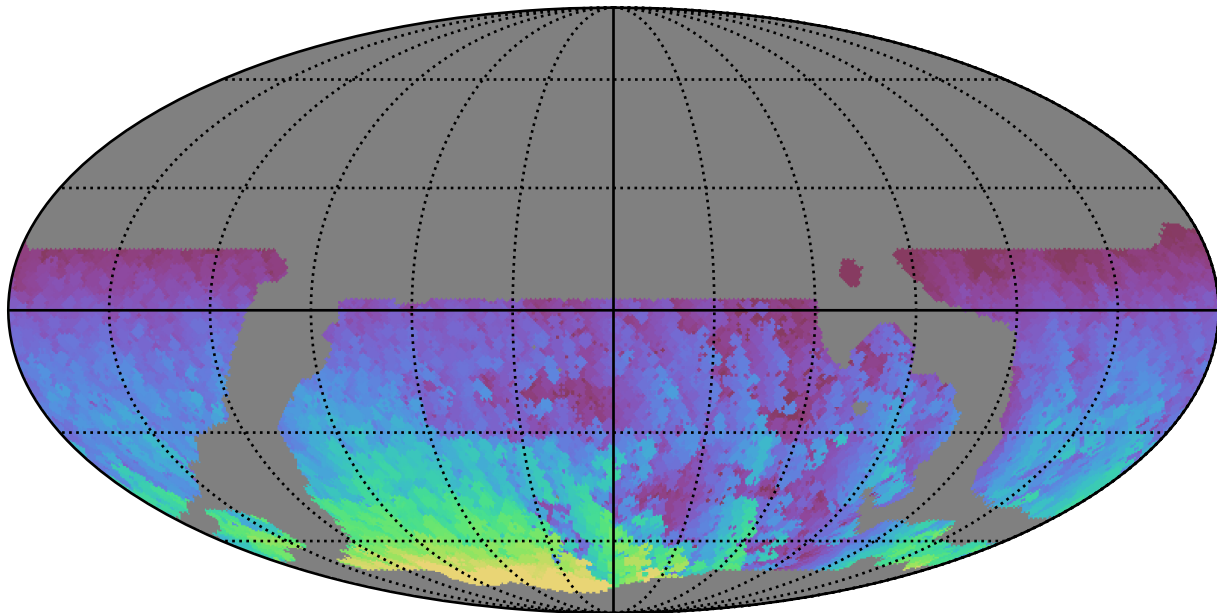
weather_cloudso12v3.4_10yrs WFD y band: Max HA
