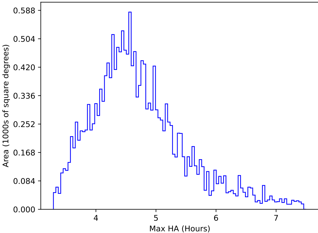
weather_cloudso12v3.4_10yrs WFD y band: Max HA
