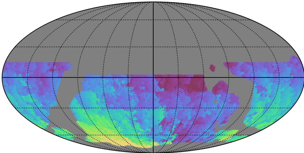
weather_cloudso12v3.4_10yrs WFD u band: Max HA
