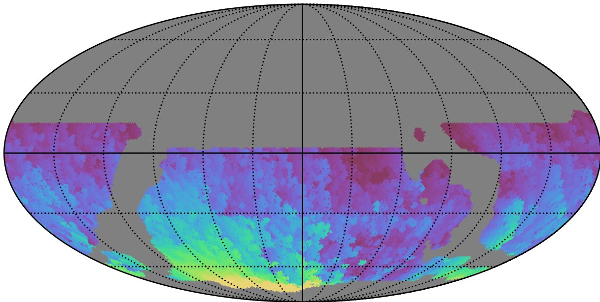
weather_cloudso12v3.4_10yrs WFD r band: Max HA
