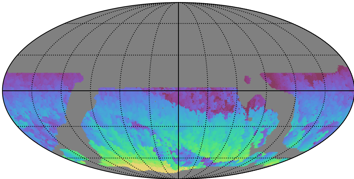
weather_cloudso12v3.4_10yrs WFD i band: Max HA
