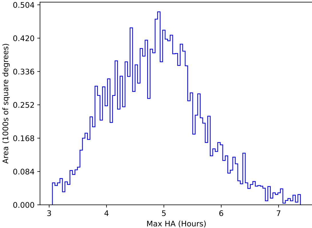
weather_cloudso12v3.4_10yrs WFD i band: Max HA
