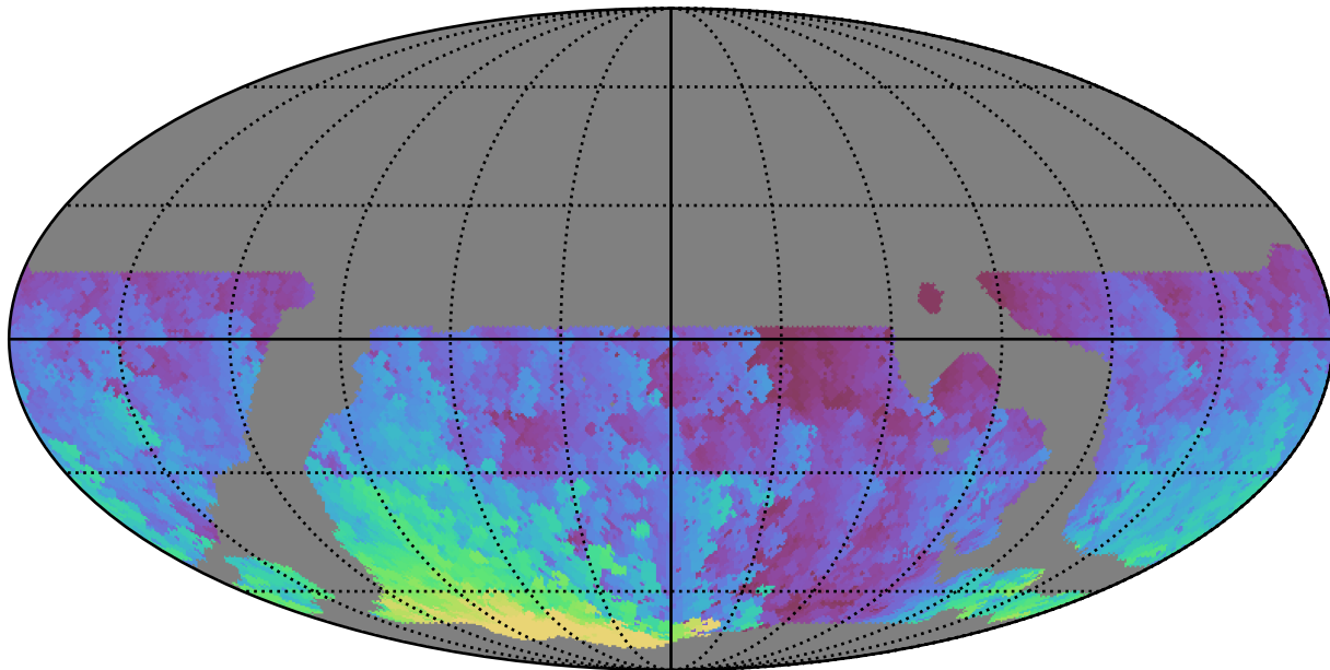
weather_cloudso12v3.4_10yrs WFD g band: Max HA
