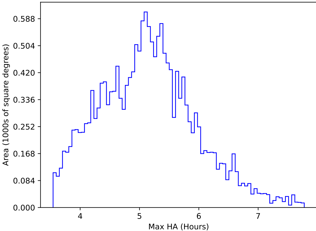
weather_cloudso12v3.4_10yrs WFD all bands: Max HA
