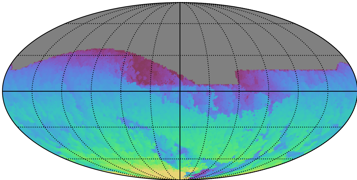
weather_cloudso12v3.4_10yrs All sky z band: Max HA
