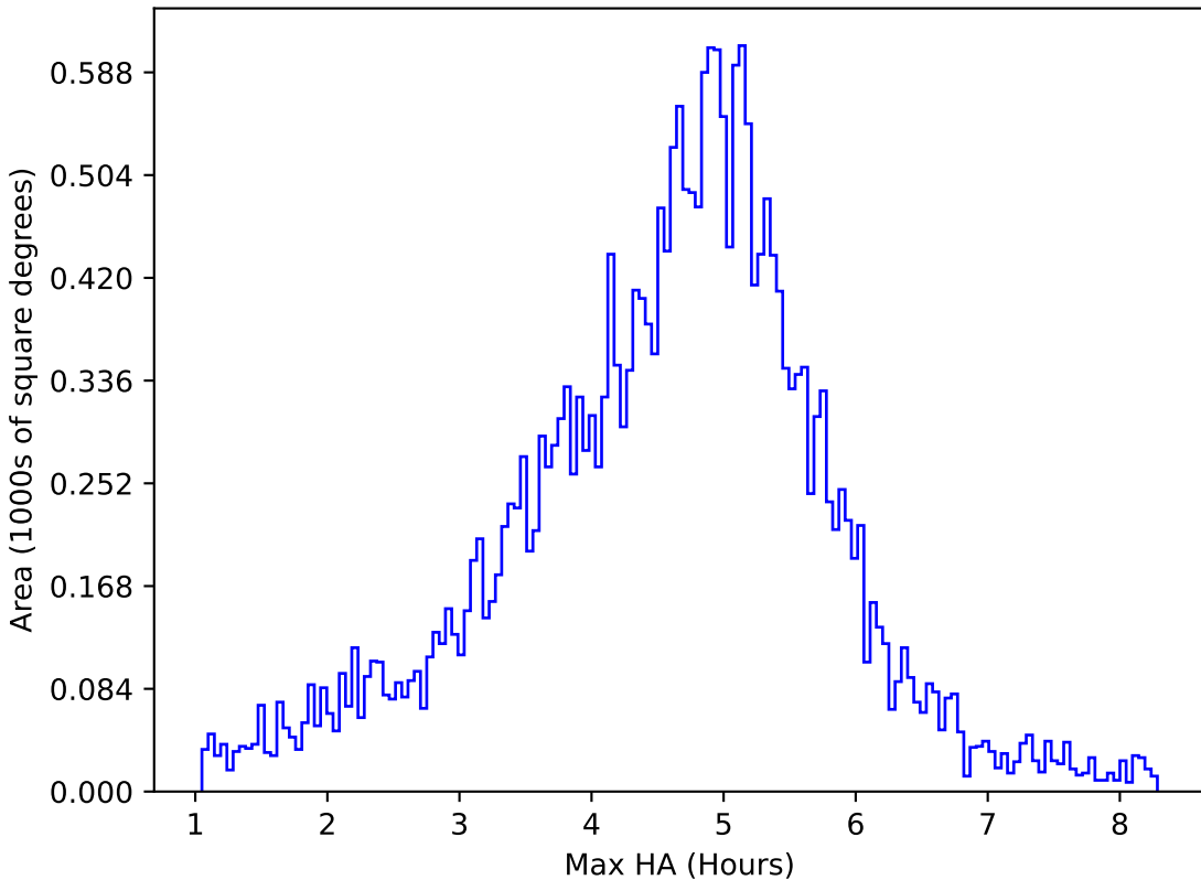
weather_cloudso12v3.4_10yrs All sky z band: Max HA
