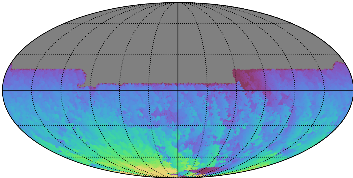
weather_cloudso12v3.4_10yrs All sky y band: Max HA
