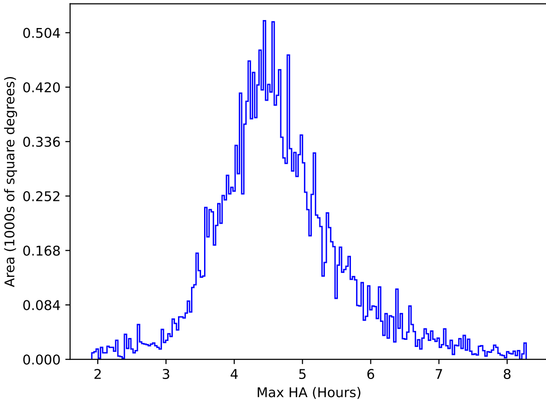
weather_cloudso12v3.4_10yrs All sky y band: Max HA
