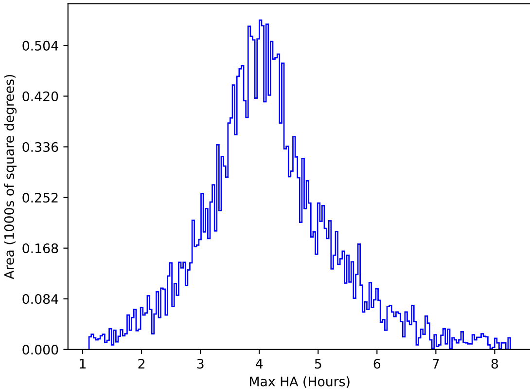
weather_cloudso12v3.4_10yrs All sky r band: Max HA
