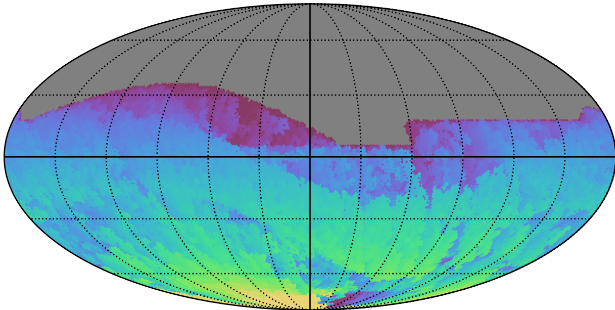
weather_cloudso12v3.4_10yrs All sky i band: Max HA
