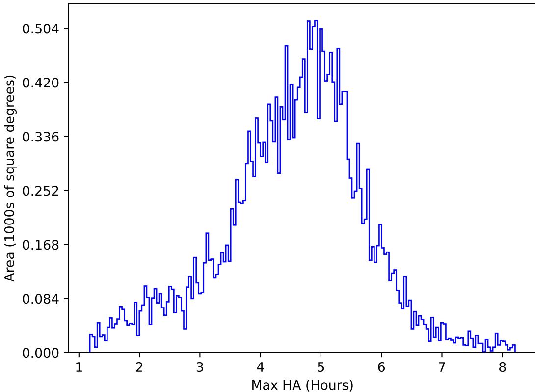
weather_cloudso12v3.4_10yrs All sky i band: Max HA
