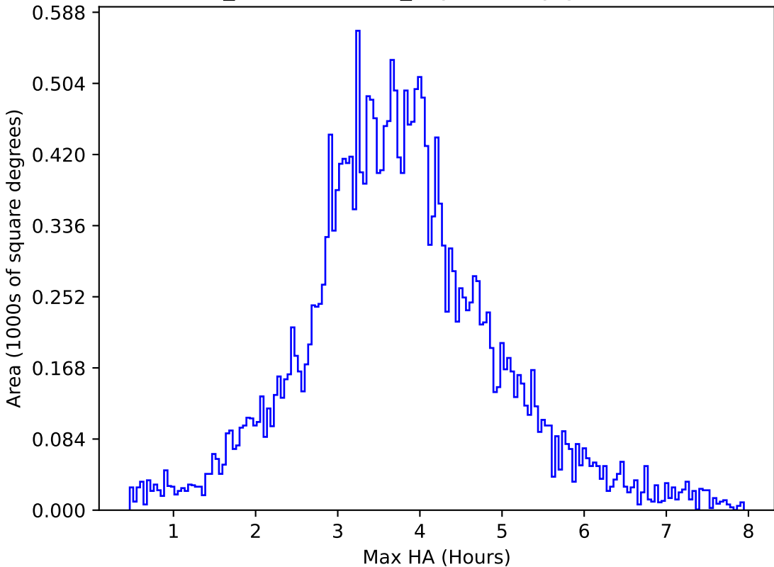
weather_cloudso12v3.4_10yrs All sky g band: Max HA
