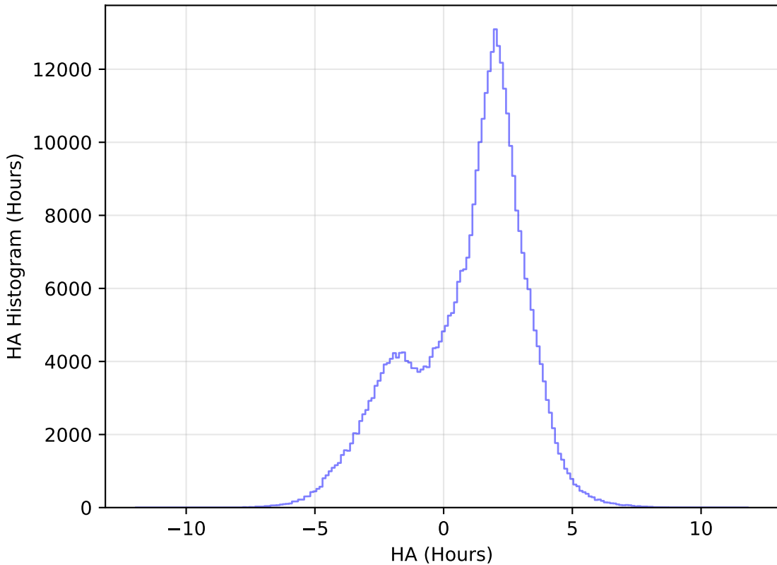
weather_cloudso12v3.4_10yrs WFD y band: HA Histogram
