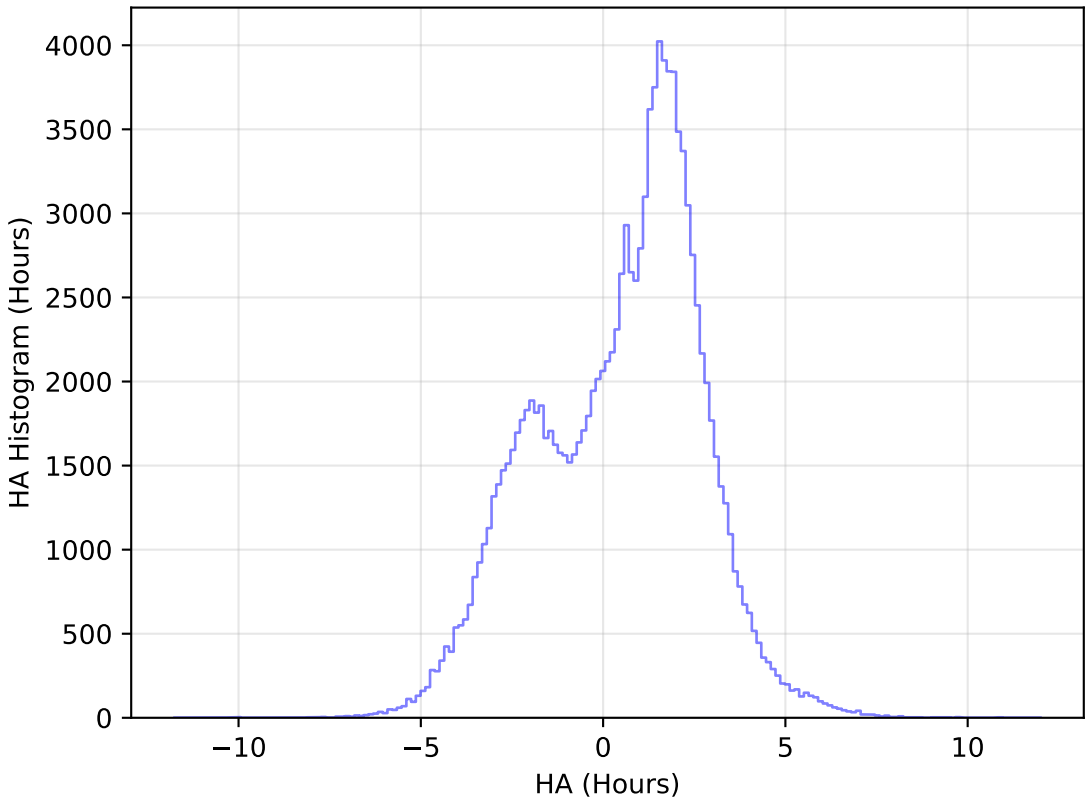
weather_cloudso12v3.4_10yrs WFD u band: HA Histogram
