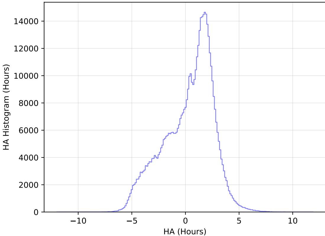
weather_cloudso12v3.4_10yrs WFD r band: HA Histogram
