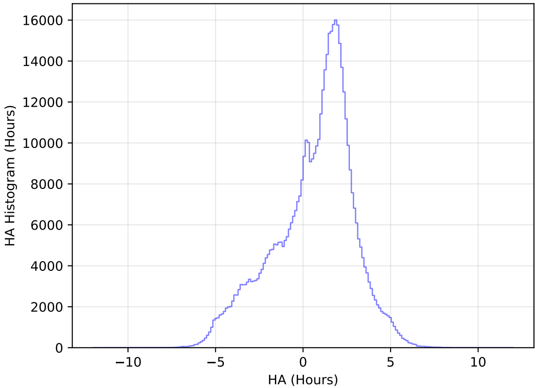
weather_cloudso12v3.4_10yrs WFD i band: HA Histogram
