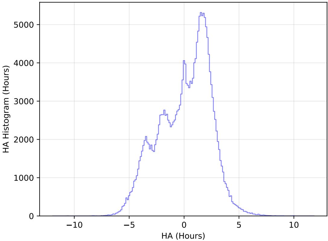
weather_cloudso12v3.4_10yrs WFD g band: HA Histogram
