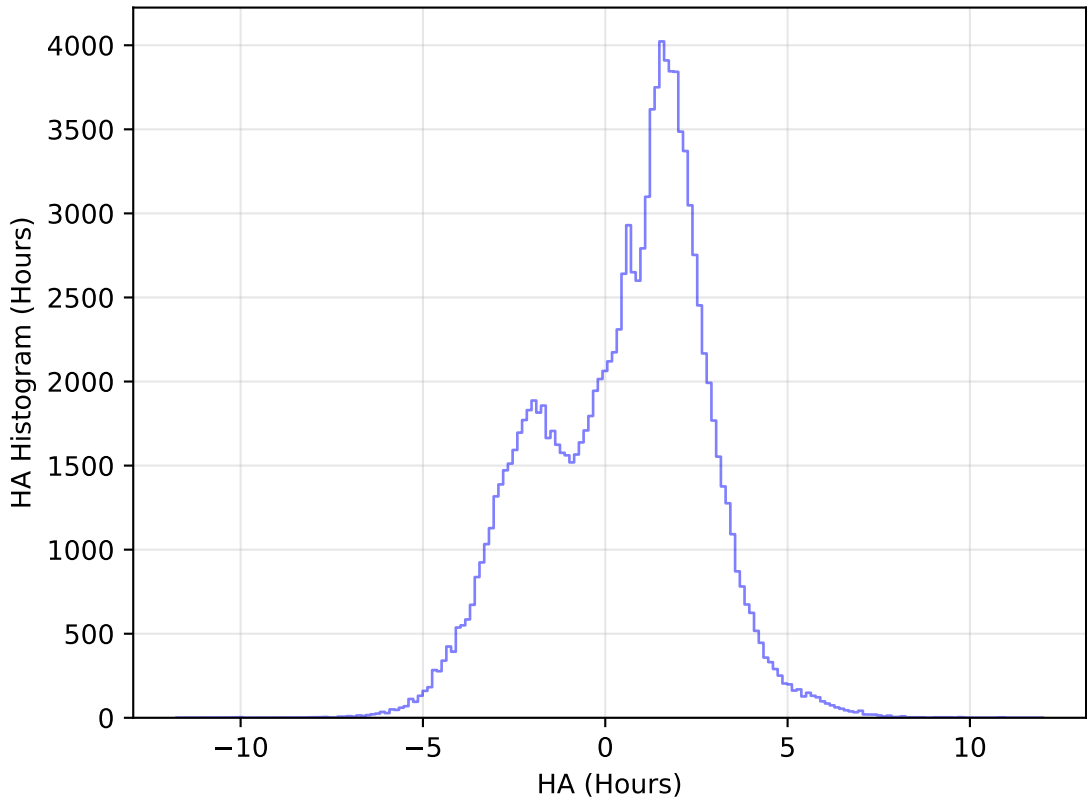
weather_cloudso12v3.4_10yrs All sky u band: HA Histogram
