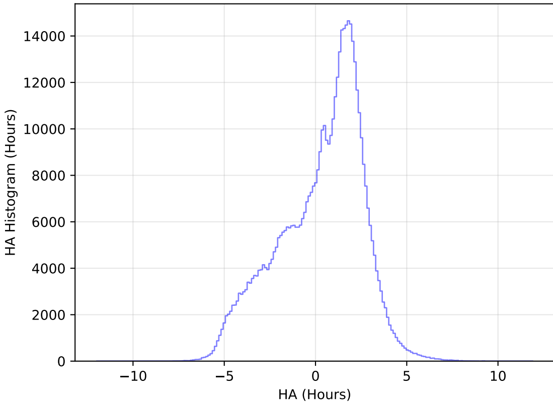
weather_cloudso12v3.4_10yrs All sky r band: HA Histogram
