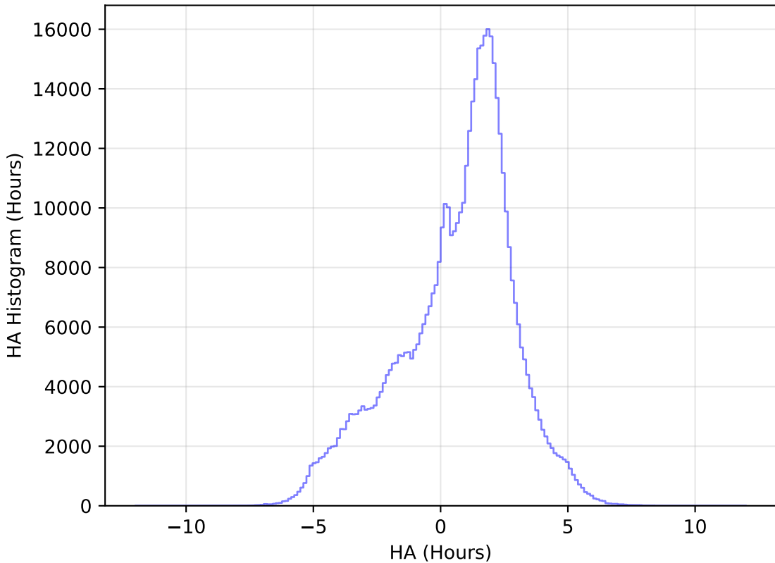
weather_cloudso12v3.4_10yrs All sky i band: HA Histogram
