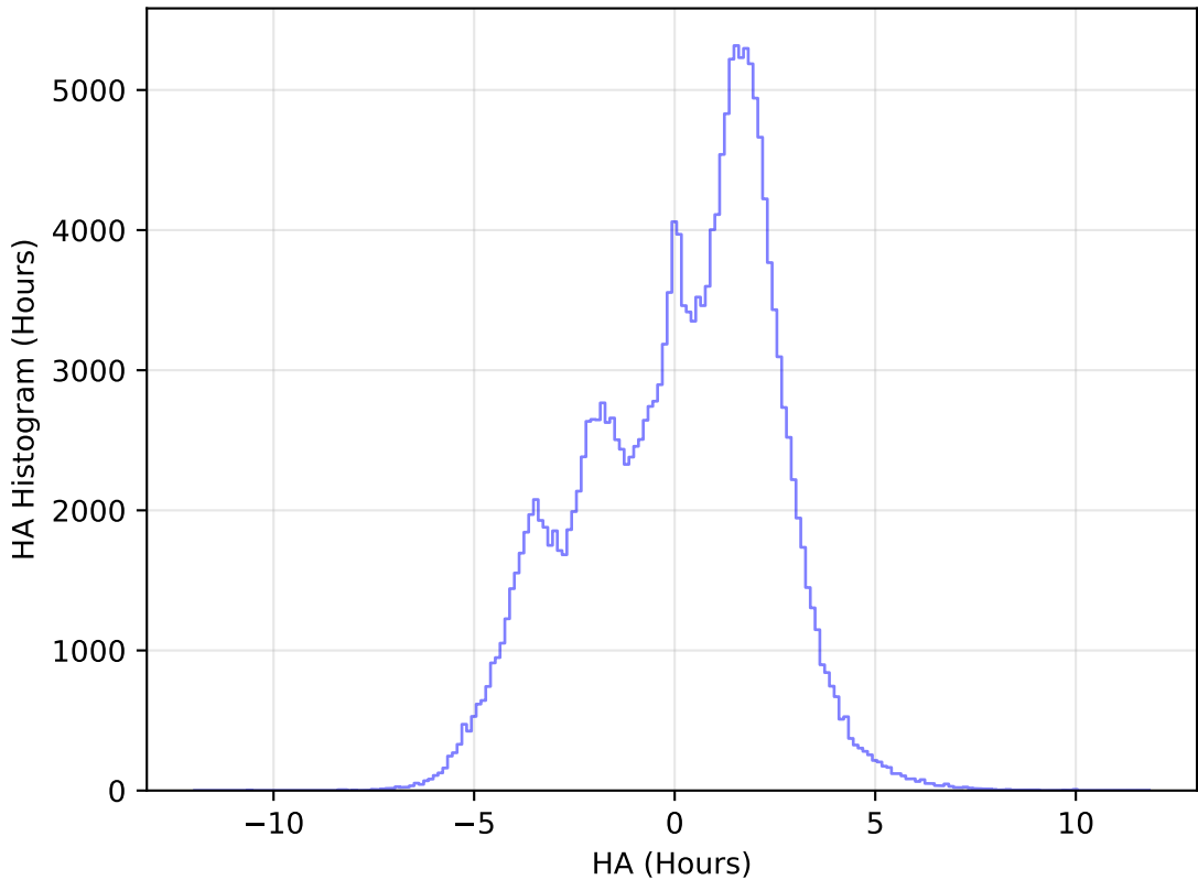
weather_cloudso12v3.4_10yrs All sky g band: HA Histogram
